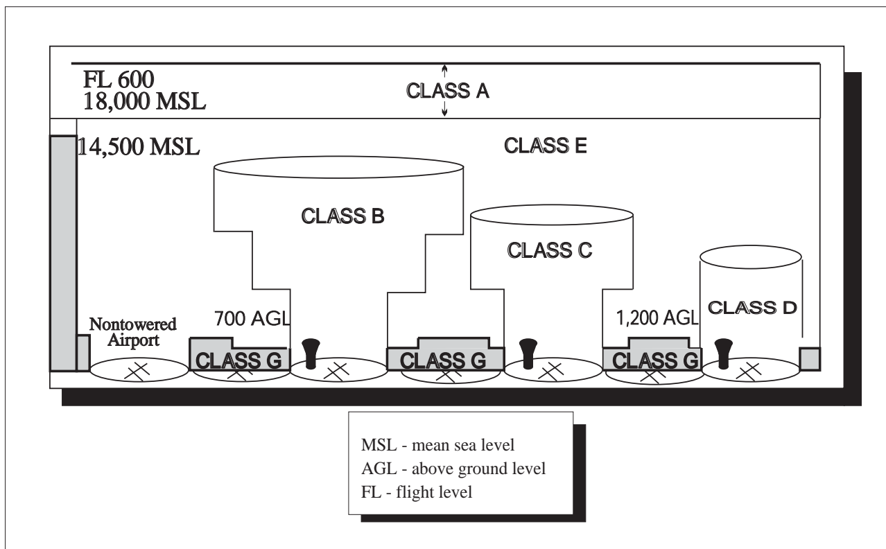
FIG 3-2-1 Airspace Classes
